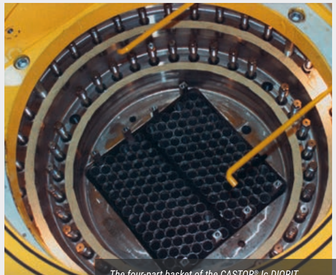
The four-part basket of the CASTOR® Ic DIORIT.
